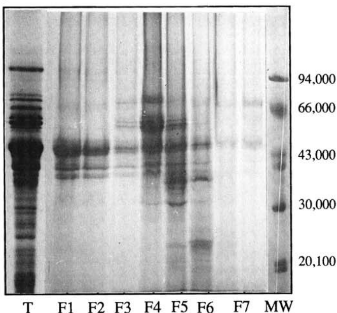
Fig. 2. Sodium dodecyl sulfate-polyacrylamide gel electrophoresis patterns of unreduced (A) and reduced (B) protein fractions (F1-F7) collected from size-exclusion high-performance liquid chromatography. T = total reduced proteins; MW = molecular weight standards.
