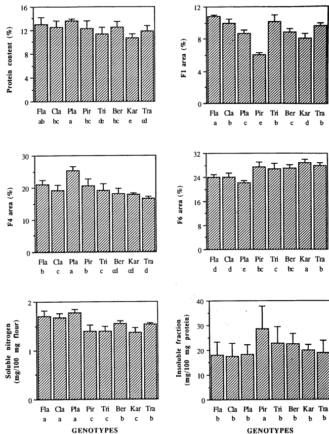
Fig. 4. Main effect of genotype as determined by the Newman-Keul homogeneity test for: protein content; percentage of chromatographic fractions F1, F4, and F6; soluble nitrogen; and insoluble residue. Fla = Flamenco, Cla = Clarine, Pla = Plaisant, Pir = Pirate, Tri = Triumph, Ber = Bérénice, Kar = Karl, Tra = Traill. Mean values with the same letter are not significantly different for each characteristic. Vertical bars represent standard deviation from means.
