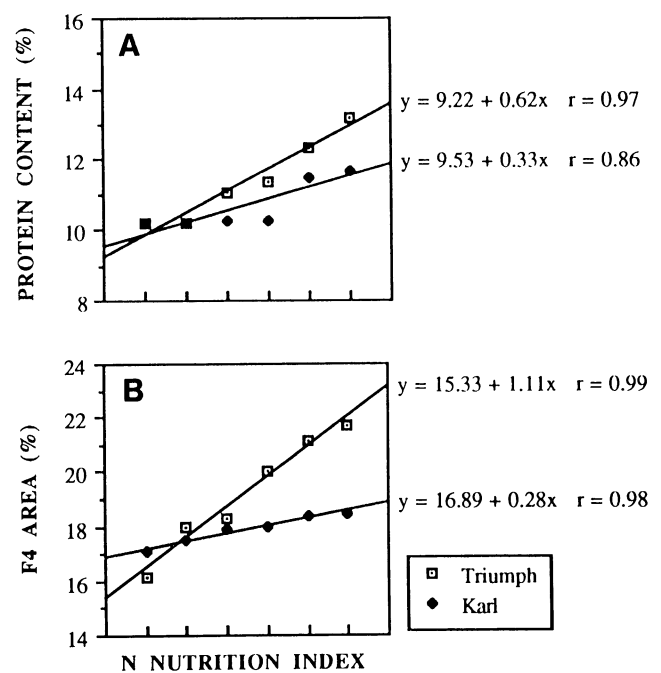
Fig. 5. Correlation with nitrogen nutrition index. (A) grain protein content (db). (B) F4 area (%).
