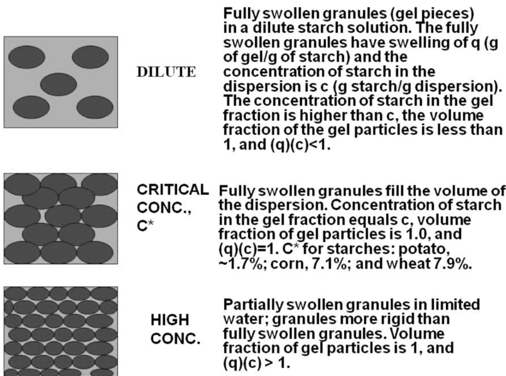
Fig. 1. Composite structure of wheat starch granules heated in water (Ring 1985; Steeneken 1989).
